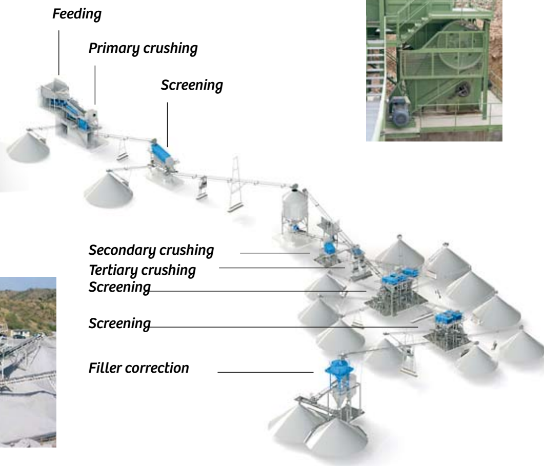
Stationary Plants
